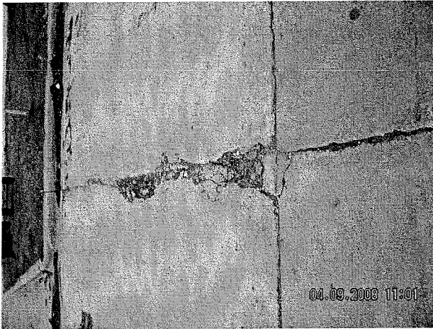
Photo of spalling at a rigid (Portland Cement-Concrete) joint
