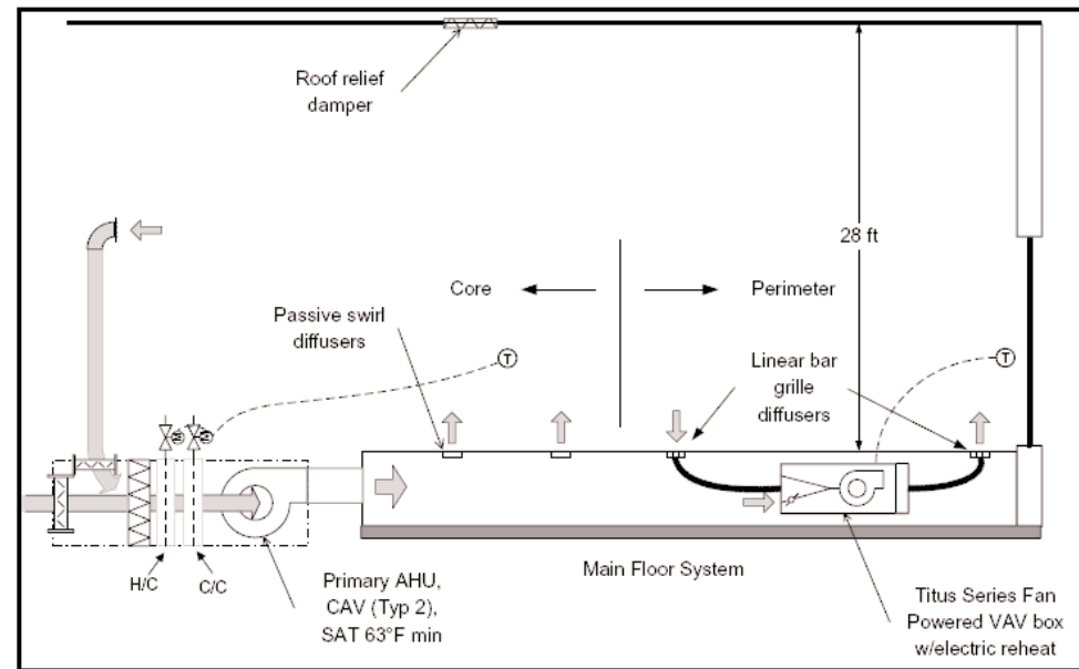
"Underfloor Air Distribution System," Tom Weber, U. of California Lawrence Berkeley National Laboratory, 2004
